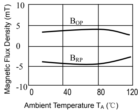
B OP and B RP VS Temperature
